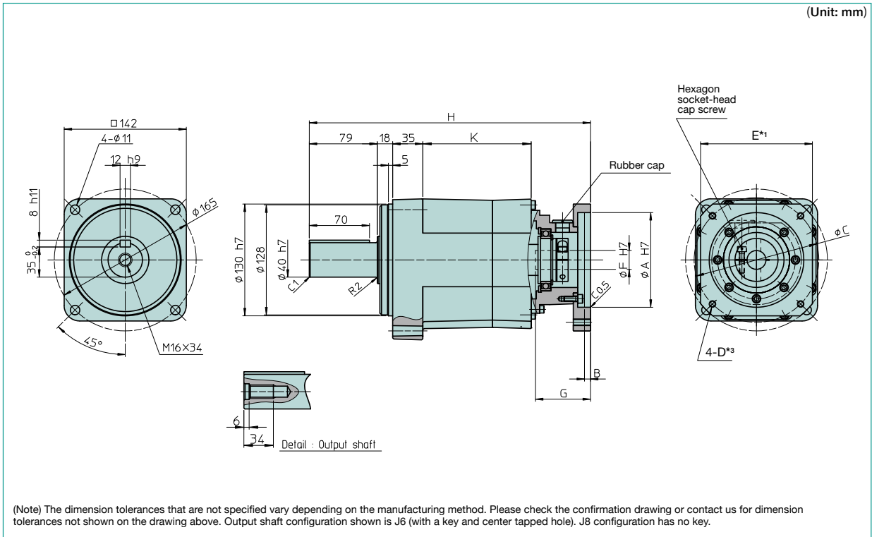
Figure 070-1 (Unit: mm)
