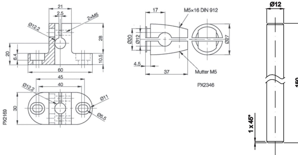
Mounting kit
