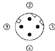
M12 4-pole Ethernet
