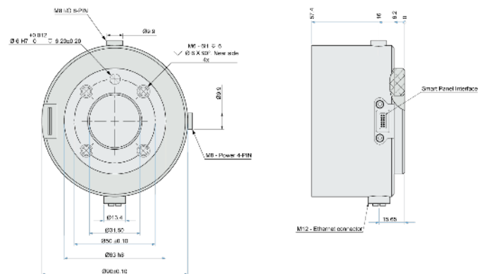
Tool flange for UR18g-950
